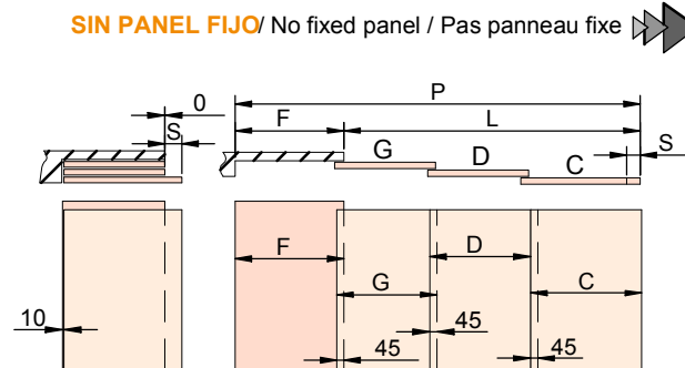
INSTALACIÓN SOLAPADA / Overlap assembly / Mountage Sournois
