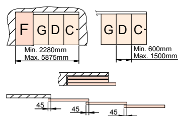
SOLAPADO / Overlap / Sournois
