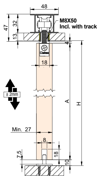
PERFIL STAR FTI FALSO TECHO INVISIBLE Star Track FTI False Ceiling Invisible
